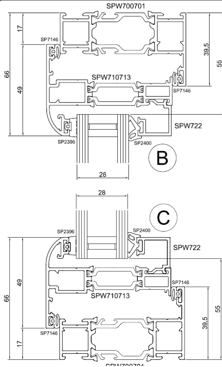
Figure 3 – Vertical section
